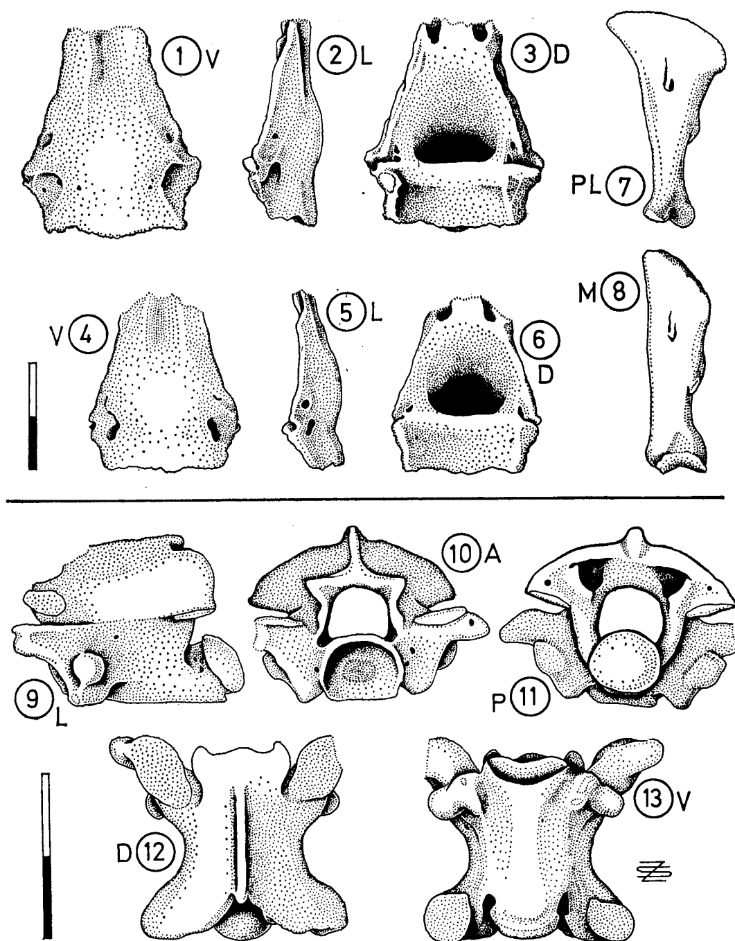
Fig. 5.— Hispanophis coronelloideus gen. sp. nov. 1-3, holotype basiparasphenoid (MNCN, no Alg I - 27); 4-6, paratype basiparasphenoid (MNCN, no Alg I - 28); 7, 8, left quadrate (MNCN, no Alg I - 29); 9-13, mid-trunk vertebra (MNCN, no Alg I - 30). A - anterior, D - dorsal, L - lateral, M - medial, P - posterior, PL - postero-lateral, V - ventral views. Scale equals 2 mm.
