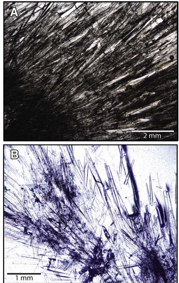
Fig. 3. Thin-section microphotographs with plain-polarized light. (A) Aragonite speleothem almost completely micritized. Micrite has a dark opaque colour whereas the primary crystals are transparent and clean. (B) Branching speleothem. Micrite appears especially in the nucleus of the fans forming dark opaque areas. (For interpretation of the references to colour in this figure legend, the reader is referred to the web version of this article.)
