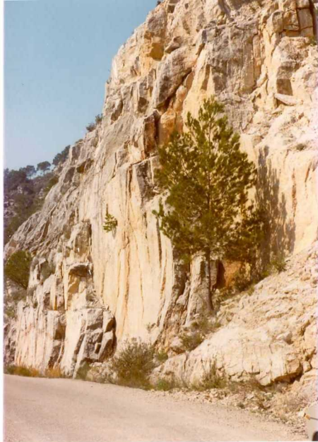
32-17-FI-OG-49 . - Muschelkalk superior ( T_{G23} ).
