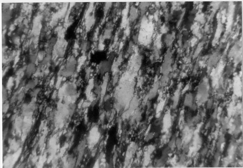
0708-IM-FR-0091.-Cuarcita esquistosa . LPx2 , Q 78 .
