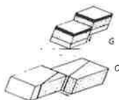
Faults: G: Normal D: Strike-Slip
